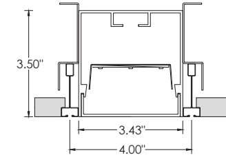
9ST - 9/16" SLOT TEE TEGULAR / 4" TECH ZONE
