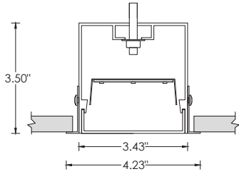
RECOMMENDED CEILING OPENING 3.75"
