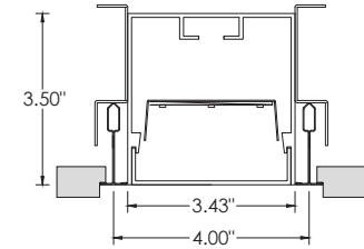
9TG - 9/16" TEGULAR
