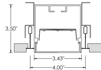
9TP - 9/16" TEGULAR
