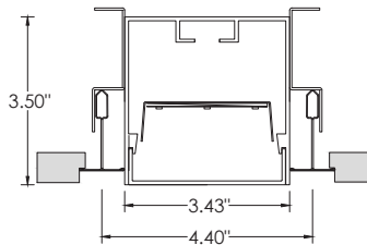
15TP - 15/16" TEGULAR
