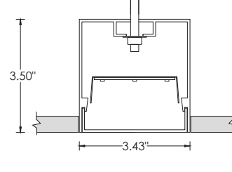
RECOMMENDED CEILING OPENING 3.49"
