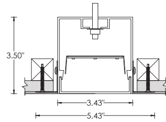
RECOMMENDED CEILING OPENING 3.93"
