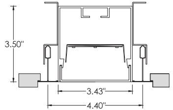
15TG - 15/16" TEGULAR
