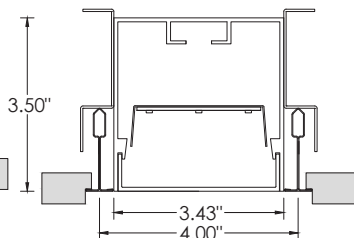
9TG - 9/16" TEGULAR
