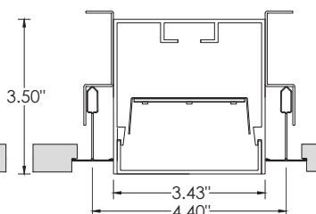
15TP - 15/16" TEGULAR
