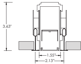
9TP - 9/16" TEGULAR
